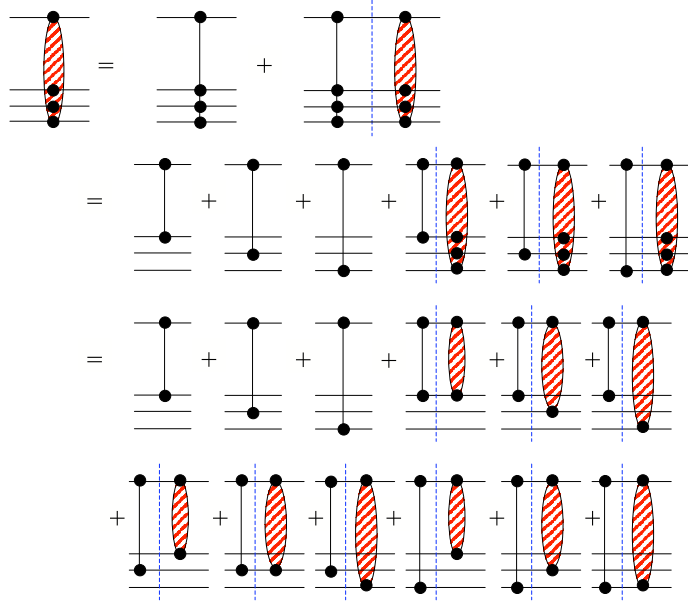
Figure 3. Diagram of the Lippman-Schwinger equation and its expansion,
