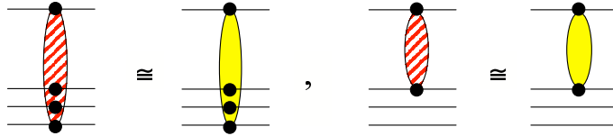
Figure 6. Diagram of the single scattering approximation T \approx \sum_{i=1}^A t_{0i} (left diagram) or the i^{\text{th}} term T_{0i} \approx t_{0i} (right diagram).
