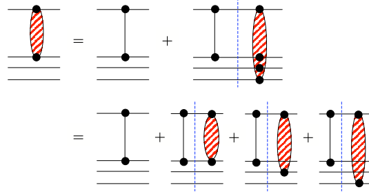
Figure 4. Diagram of the i^{\text{th}} term of the Lippman-Schwinger equation and its expansion, T_{0i} = v_{0i} + v_{0i}G_0T = v_{0i} + v_{0i}G_0 \sum_j T_{0j}
