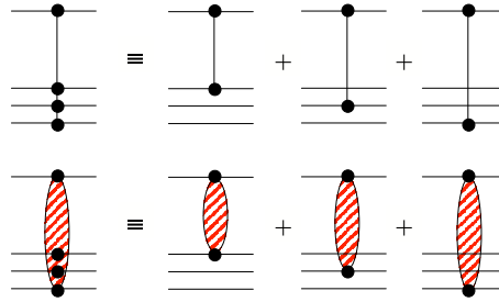
Figure 1. Diagrams of the definitions V \equiv \sum_{i=1}^A v_{0i} (top) and T \equiv \sum_{i=1}^A T_{0i} (bottom) for a target containing 3 particles.
