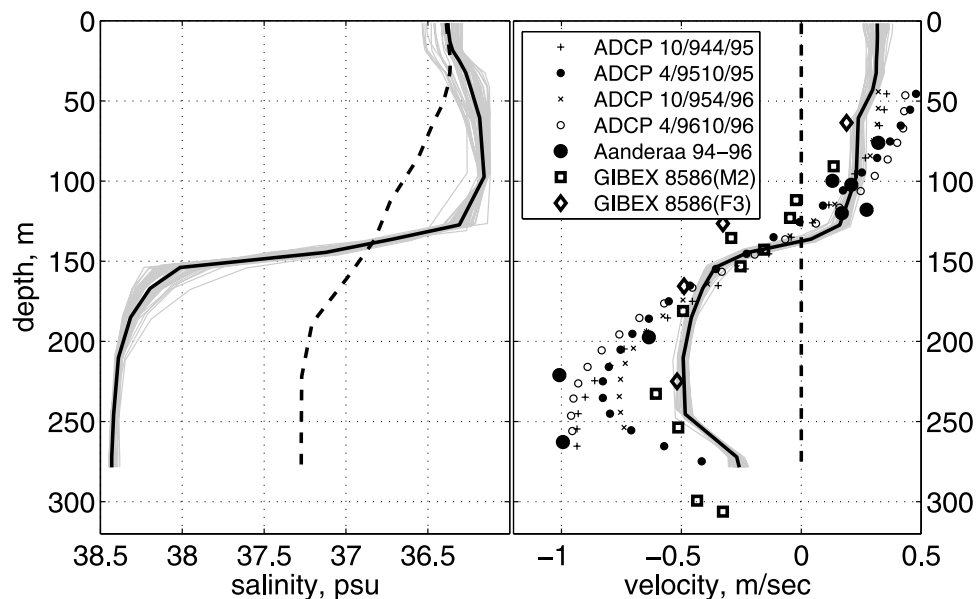
Figure 3. Simulated vertical profiles of (left) salinity and (right) horizontal velocity in the Strait of Gibraltar near the Camarinal Sill ( 5.72^\circ\text{W} , 35.9^\circ\text{N} ). The thick dashed lines are the initial profiles; the thin gray lines are simulated profiles for every 3 days, and the thick solid lines represent the time-averaged profile. The observed velocity profiles are adapted from Figure 5.7.5 of Candela [2001].
