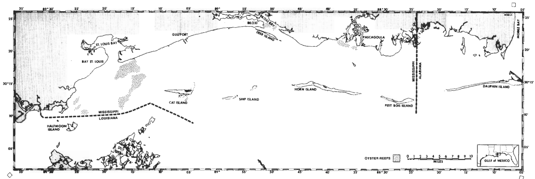
Figure 1. Location of productive natural oyster reefs, Mississippi Sound.
