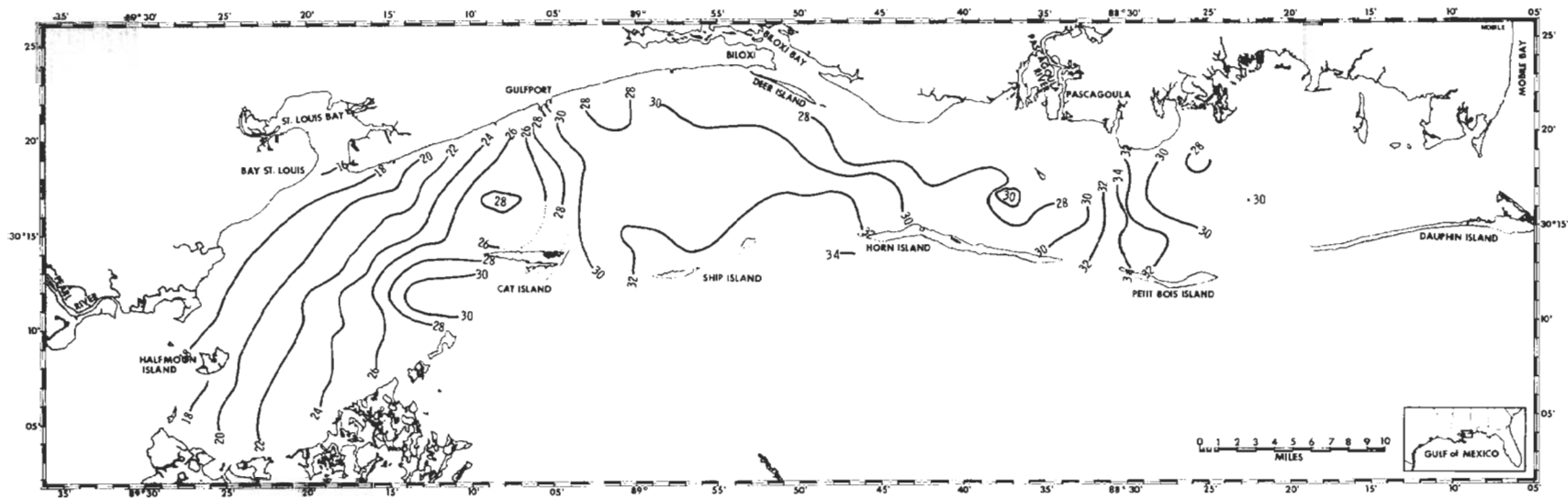
Figure 4. Distribution of maximum levels of salinity (ppt), Mississippi Sound, 1973-1975.
