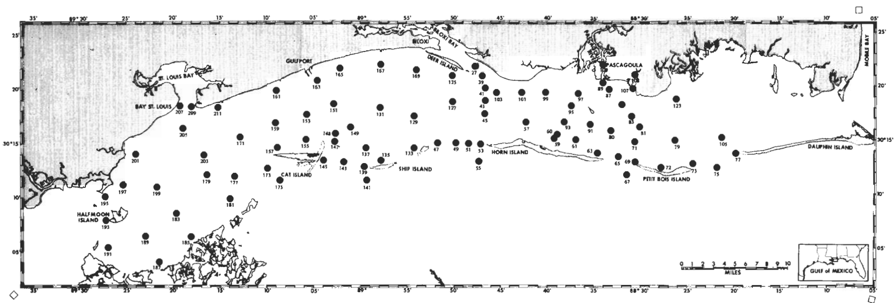
Figure 2. Station Locations, Mississippi Sound area.
