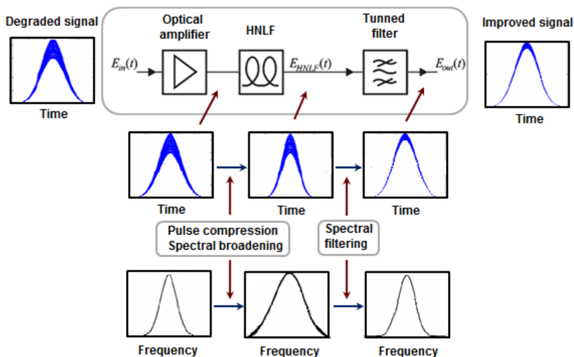
Figure 3-12: Configuration and operating principle of the first-type regenerator.
