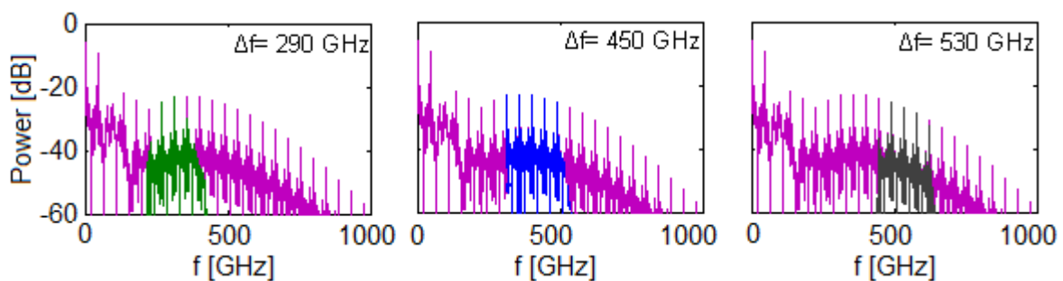
Figure 3-31: Spectrum filtering; in purple the broaden signal due to \varphi_{NL} , in green, blue, and grey the BW filtered.
