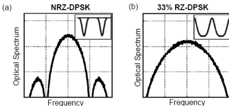
Figure 2-6: DPSK spectra and eye diagrams of (a) NRZ-DPSK and (b) RZ-DPSK
