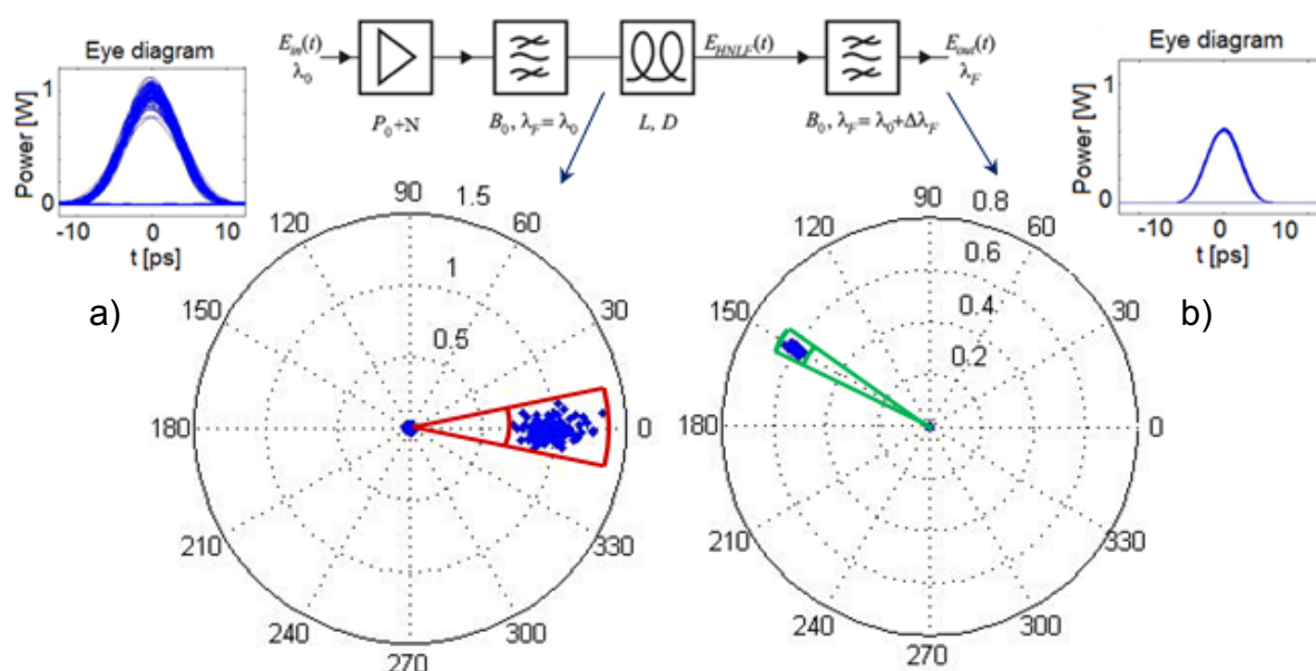
Figure 3-16: Eyediagrams and module/phase polar plots of the signal before (a) and after (b) being regenerated
