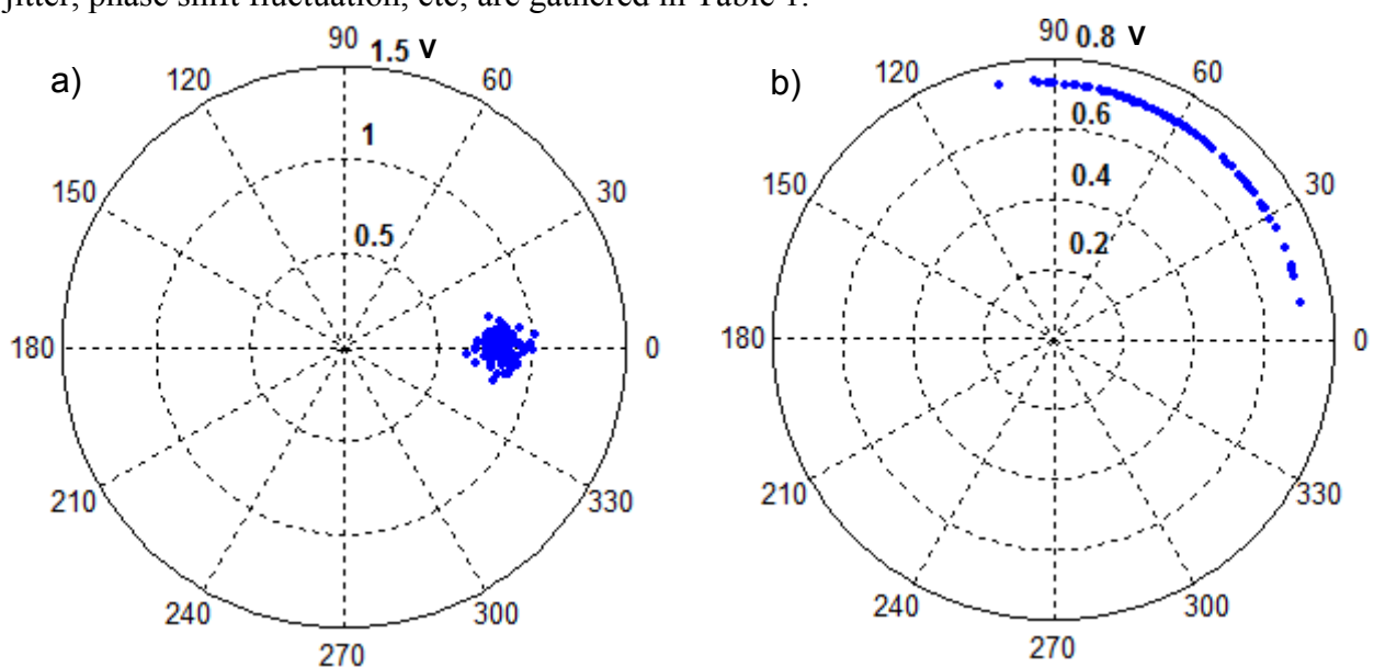
Figure 3-3: Characteristic diagrams, using polar coordinate system, of the NRZ-DSPK module/phase before (a), and after (b) the regenerator.
