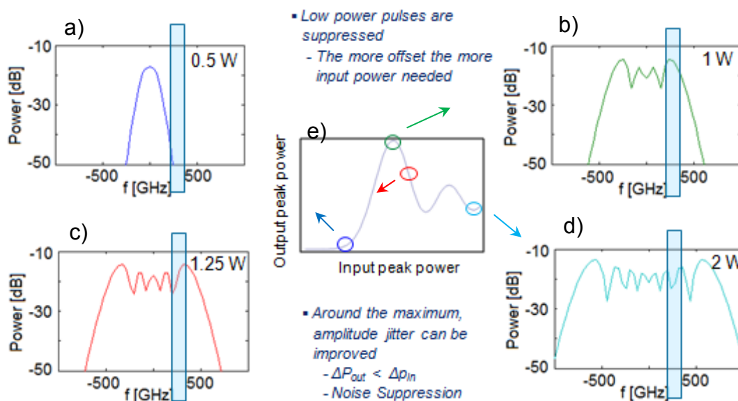
Figure 3-14: In order to understand the power transfer function response (e), spectrums corresponding to different input power are depicted, maintaining L \cdot \gamma = 4\pi , offset=300GHz, bandwidth=1/T 0 =150GHz.
