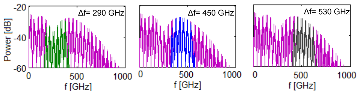
Figure 3-23: Spectrum filtering; in purple the broadened signal due to \phi_{NL} , in green, blue, and grey the BW filtered respectively.
