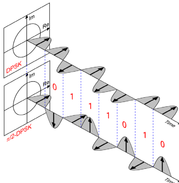
Figure 2-3: Schematic representation of the amplitude and phase evolution of DPSK (upper) and \pi/2 -DPSK (lower). Return-to-zero (RZ) pulses are used in this example. [2]
