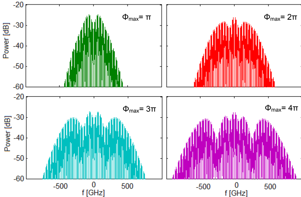
Figure 3-22: Spectrum of the signal after the Kerr medium for different values of nonlinear phase shift \phi_{MAX} .
