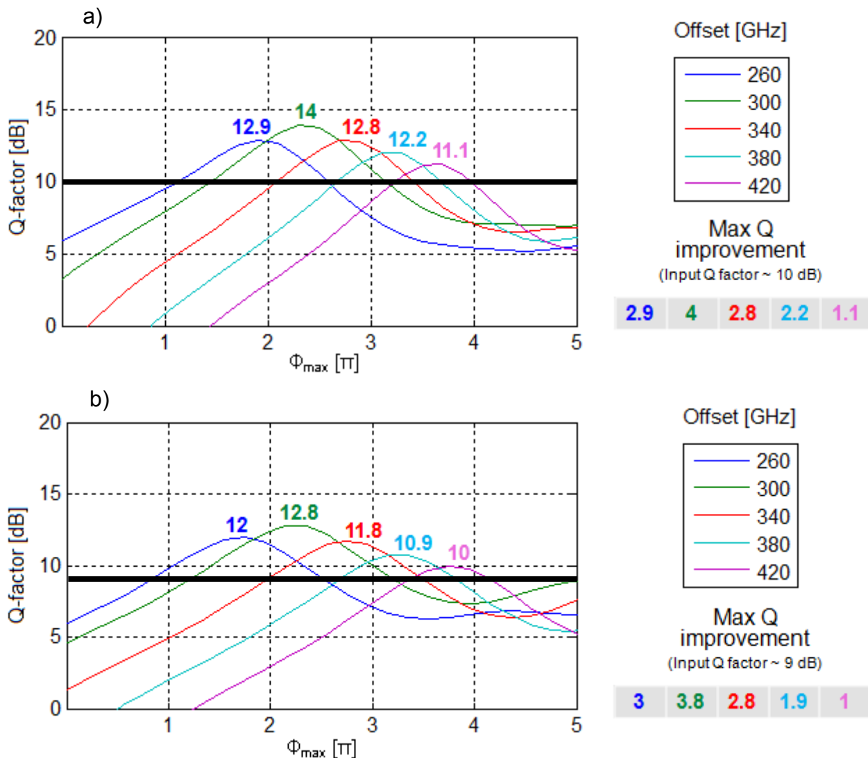
Figure 3-26: Q-factor characteristic curve in function of induced phase shift for (a) a phase amplitude depth of 0.7, and (b) 0.6.
