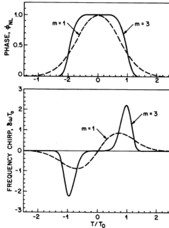
Figure 2-14: Temporal variation of SPM-induced phase shift \phi_{\text{NL}} and frequency chirp \delta\omega .
