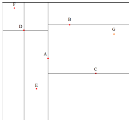
Figure 15. Example of a 3-dimensional q-kd tree
