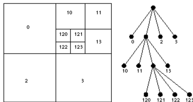
Figure 5. Region quad-tree [11]
