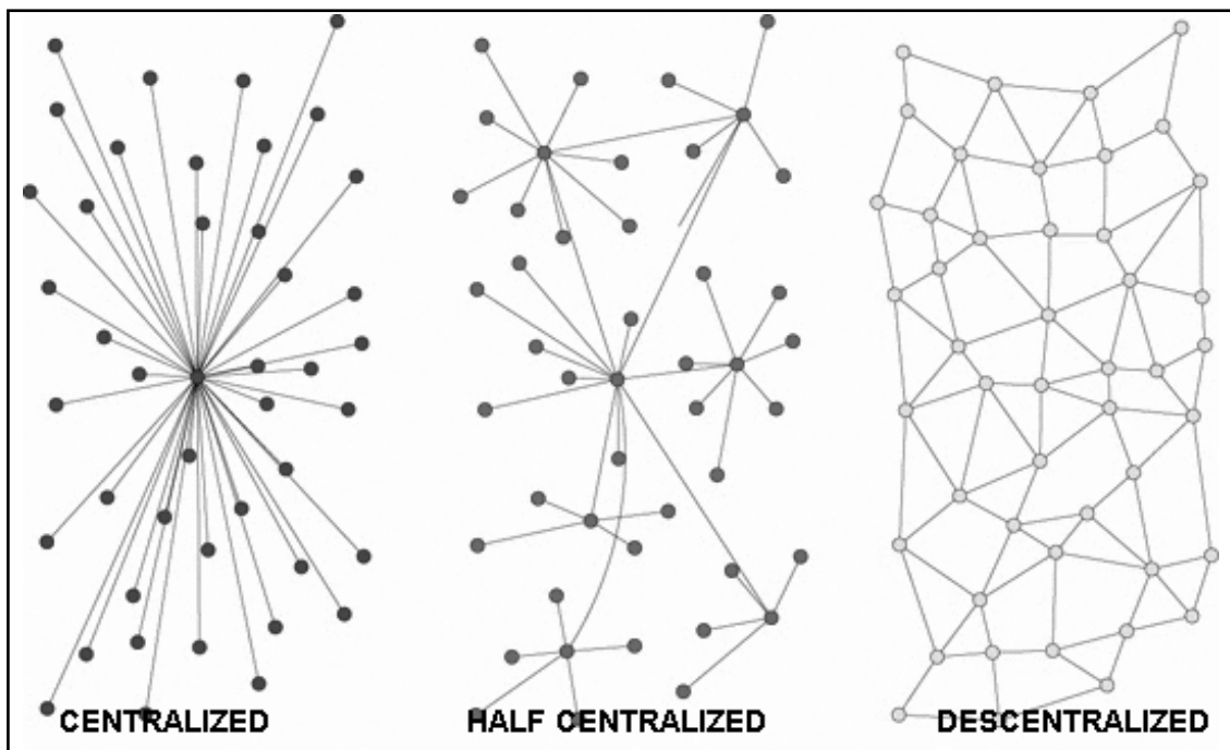
Figure 2: Network Classification
