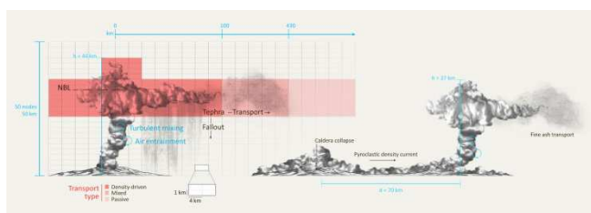
Figure 1. . Illustration of a typical multi-phase super-eruption with an initial (a) Sustained Plinian phase; followed by a (b) Caldera-collapse and large pyroclastic density currents eventually leading to secondary, co-ignimbritic plumes offset from the vent. Nodes with grey outline represent the model domain used for the CI model simulations. Our simulations used a grid spacing 0.2 degrees latitude and longitude (~4km), and 1 km cell height. Red nodes illustrate the effect of the density-current and the corresponding transport regimes in the umbrella cloud based on the best-fit model parameters (blue text) associated to the CI event.
