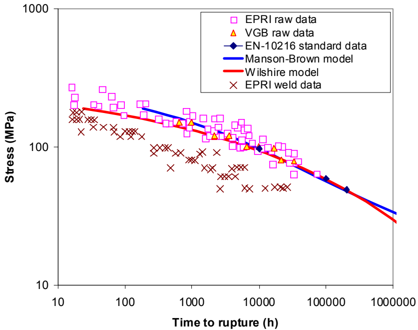
Fig. 12. EPR and VGB data for X20 steel at 600°C with time to rupture models (classical Manson-Brown and Wilshire) optimized on EN-10216 creep strength data.
