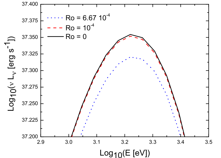
Fig. 19. Luminosity as a function of the energy for some values of R_0 > 0 , for a f(R) -Kerr black hole of angular momentum a = 0.99 .
