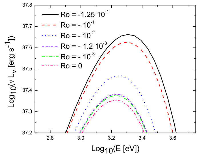
Fig. 17. Luminosity as a function of the energy for some values of R_0 < 0 , for a f(R) -Kerr black hole of angular momentum a = 0.99 .
