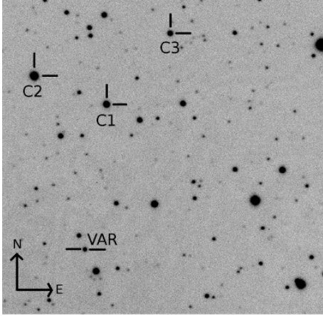
Fig. 1. One of the CCD frames obtained at Piszkestető, Konkoly Observatory, with the variable and comparison stars marked. The field of view is \approx 7' \times 7' .
