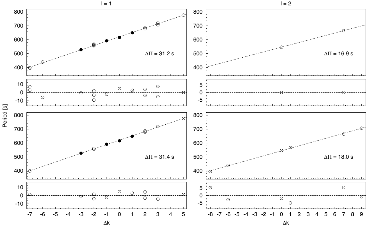
Fig. 4. Periods of Table 4 plotted in the \Delta k – period planes. Filled circles denote average periods by the 9\mu\text{Hz} spacings. The panels on the left and right show the \ell = 1 and 2 solutions and their linear least-squares fits, respectively. The residuals of the fits are also presented. Top and bottom rows display different solutions by changing some periods' presumed \ell values. The resulting period spacings ( \Delta\Pi_{\ell=1,2} ) are denoted.
