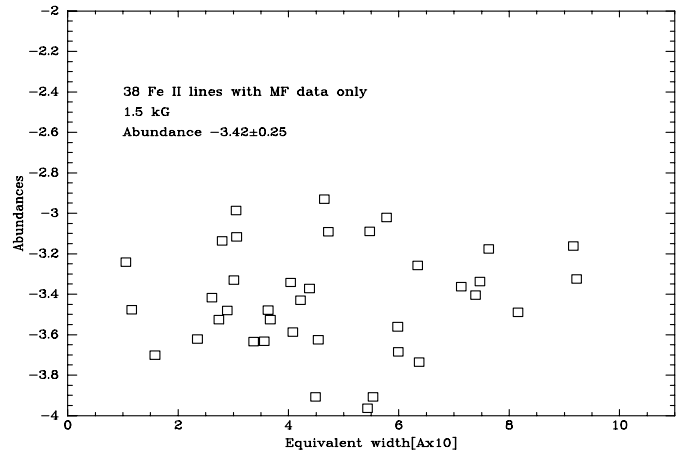
Fig. 6. Abundance vs. Equivalent width for 38 FeII lines, using only the gf values from Martin et al. (MF). The minimum scatter is obtained for a value of 1.5 kG.
