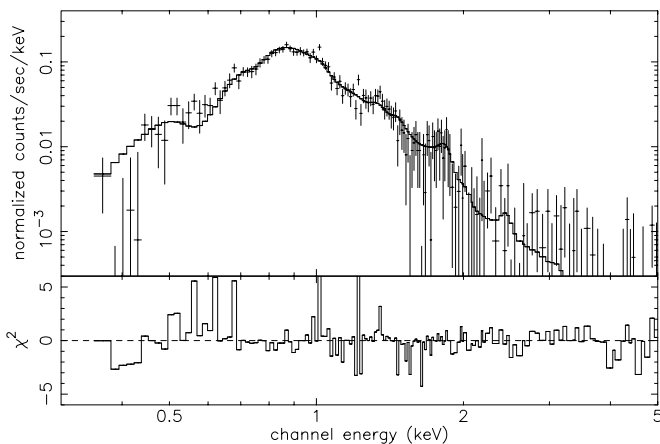
FIG. 6.— Chandra X-ray spectrum of the extended emission around HD 5980, shown along with the best-fit absorbed mekal model, with N(\text{H}) = 0.12 \times 10^{22} cm -2 , kT = 0.66 keV, and Z = 0.17 Z_{\odot} (see § 5).
