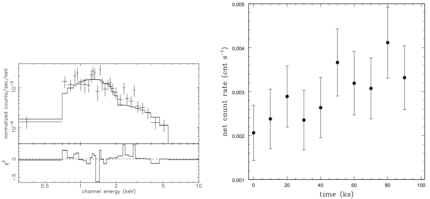
FIG. 5.—(a) Chandra X-ray spectrum of HD 5980, shown along with the best-fit absorbed mekal model, with N(\text{H}) = 0.22 \times 10^{22} \text{ cm}^{-2} and kT = 7.04 \text{ keV} . (b) The Chandra X-ray light curve of HD 5980, in the 0.3–10 keV range and with 10 bins of 10 ks each.
