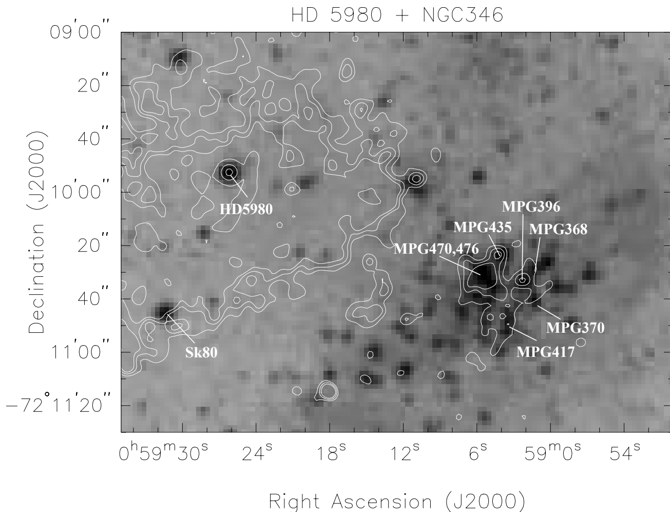
FIG. 3.— Chandra X-ray data of the NGC 346/HD 5980 region superposed on the DSS image, showing the extended nature of the X-ray source associated with the cluster. The location of the brightest stars in the cluster are indicated. The X-ray data were first binned by a factor of 2 and then smoothed by convolution with a Gaussian of \sigma = 2'' .
