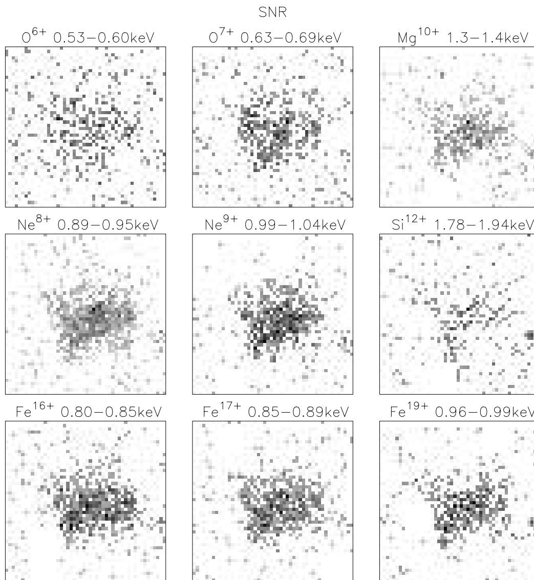
FIG. 7.—Narrowband X-ray images of the extended emission surrounding HD 5980. Each image is labeled with the principal line-emitting ion and the energy range used to generate the image.
