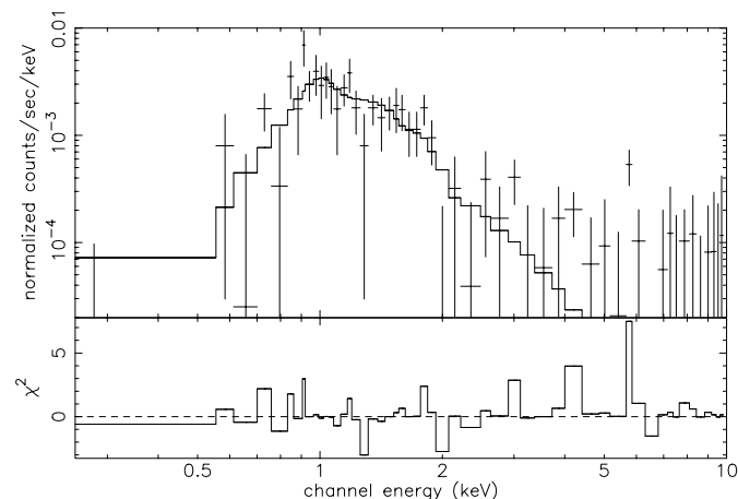
FIG. 4.—X-ray spectrum of the NGC 346 cluster, shown along with the best-fit absorbed mekal model, with N(\text{H}) = 0.42 \times 10^{22} \text{ cm}^{-2} and kT = 1.01 \text{ keV} (see § 3).
