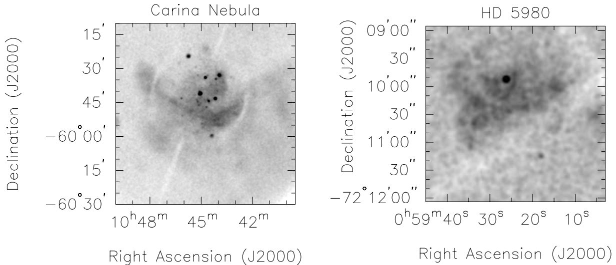
FIG. 8.—X-ray images of the Carina Nebula (24 ks; ROSAT PSPC observation 900176) compared to the extended emission around HD 5980. If we assume a distance of 2.3 kpc for the Carina Nebula and 59 kpc for the SMC, both images are \sim 55 \times 55 pc. ROSAT PSPC support rings and Chandra ACIS-I CCD gaps can be spotted on these images. Both images were smoothed by convolution with a Gaussian ( \sigma = 15'' for the Carina Nebula and \sigma = 2'' after binning by a factor of 2 for HD 5980).
