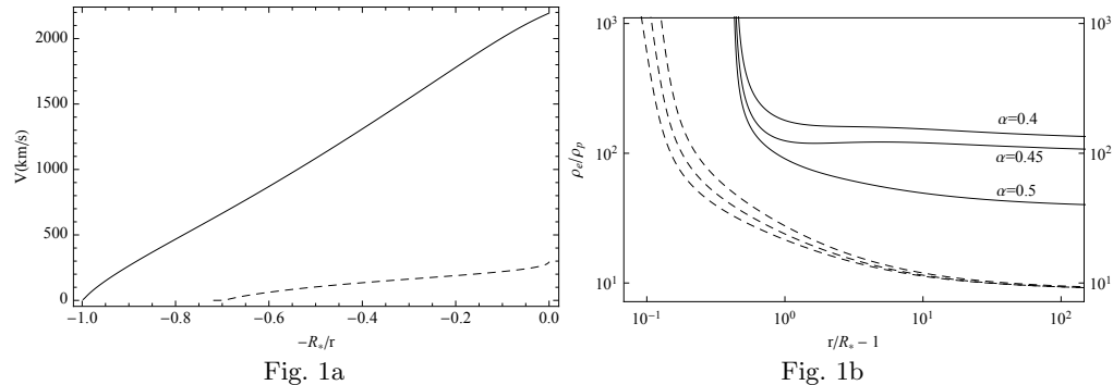
Figure 1. a) Velocity versus u for equator ( dashed line ) and pole ( solid line ) with \alpha = 0.4 and \delta = 0.07 . b) Solid lines: Density contrasts for \omega = 0.99 and \delta = 0.07 . Dashed lines: Spherical cases.
