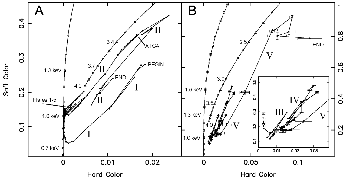
FIG. 3.—Color-color diagrams for RXTE Gain Epoch 3 (a) and Epoch 4 (b). The inset in (b) shows an enlargement of the lower left-hand part of the track in (b). Errors in (a) are omitted since they were smaller than the symbol size. The definition of the colors can be found in § 2. The squares give the expected location for a pure disk blackbody spectrum, with different temperatures as indicated, and the triangles those for a pure power-law spectrum, with different indices as indicated. The beginning and end points of the data are marked. The locations of the flares and hard branches are indicated by 1–5 and I–V, respectively. The RXTE/PCA observation taken on the day of our radio observation (MJD 51,248) is indicated in (a) by “ATCA.”
