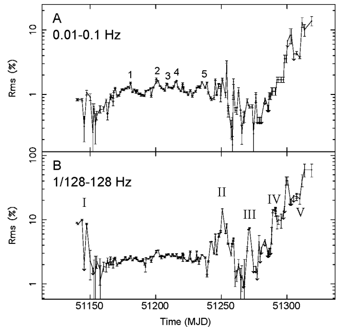
FIG. 5.—Fractional rms amplitude of 0.01–0.1 Hz noise (a) and the 1/128–128 Hz noise (b) as a function of time. Some observations were added together to obtain significant detections, and they were each plotted at their combined value. Upper limits are depicted by small arrows. Flares are labeled 1–5 in (a) and branches I–V in (b).
