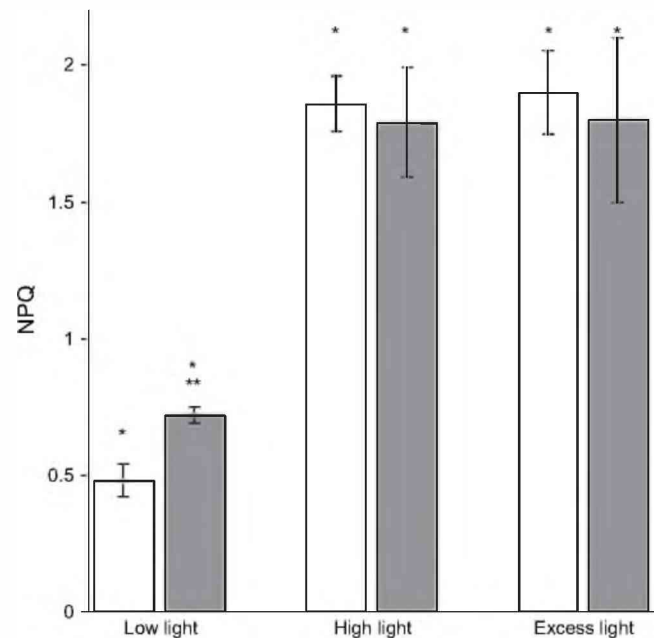
Fig. 7. Changes in non-photochemical quenching ( NPQ ) in leaves of wheat plants subjected to drought and treated with SHAM (grey bars). White bars represent drought-exposed leaves incubated without SHAM. One asterisk indicates significant difference from well-irrigated plants at an identical light regime (ANOVA, P \leq 0.05 ). Two asterisks indicate significant differences from droughted plants in the absence of SHAM, at an identical light regime (ANOVA, P \leq 0.05 ). Each value represents the mean \pm SD (vertical bars) of four independent experiments.
