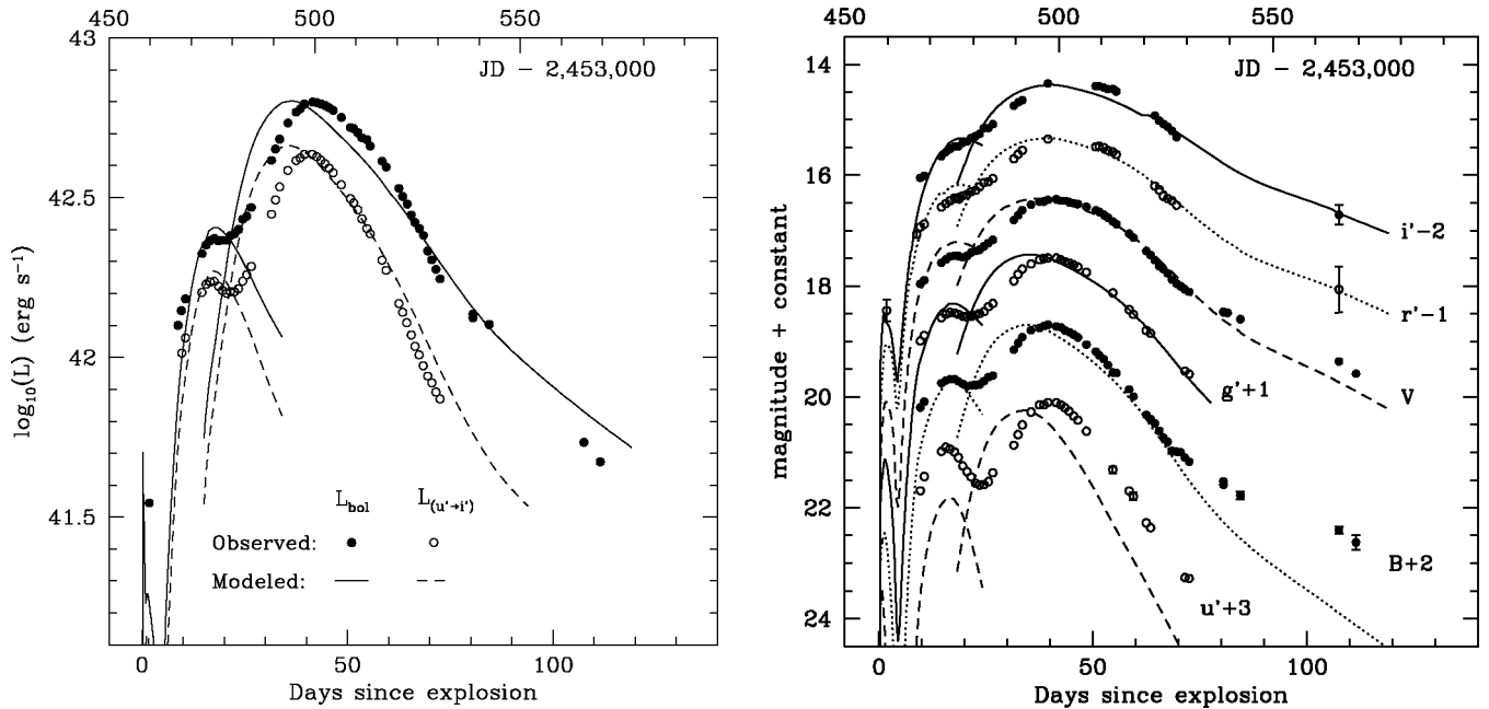
FIG. 11.— Left : Bolometric ( solid line ) and UVOIR ( dashed line ) luminosities of a composite model made of two explosions: (a) the 2 \times 10^{51} ergs explosion of 1.72 M_{\odot} of helium and heavy elements containing 0.1 M_{\odot} of ^{56}\text{Ni} , and (b) the 2 \times 10^{51} ergs explosion of an 8.29 M_{\odot} WN star. Neither model had mixed ^{56}\text{Ni} . The time of outburst was assumed to be JD 2,453,458. Component a is observable until about 20 days after outburst, when it is overrun by component b. Right : Contributions of components a and b to the u'g'r'i'BV light curves ( lines ) compared with the observations ( circles ).
