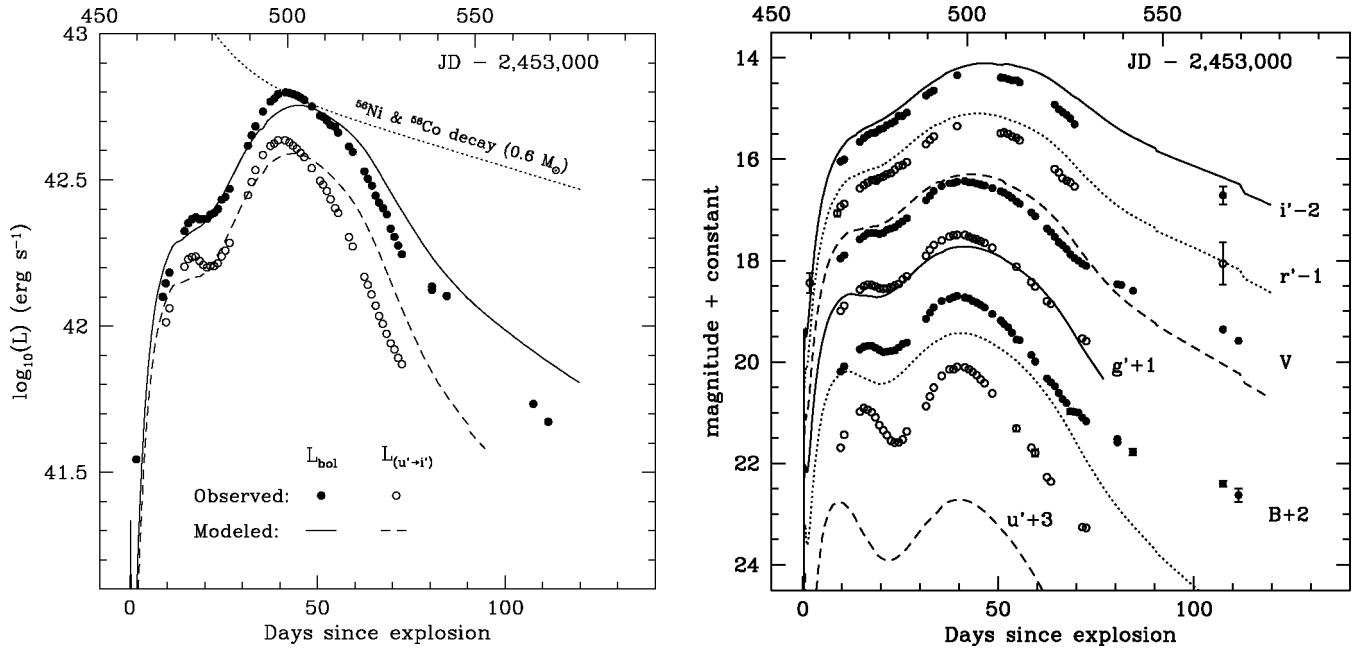
FIG. 10.— Left : Modeled bolometric ( solid line ) and UVOIR ( dashed line ) luminosities of the mixed 8.29 M_{\odot} WN star explosion. The circles mark the UVOIR luminosity L_{u' \rightarrow i'} ( open ) and the bolometric luminosity L_{\text{bol}} ( closed ), as derived from the observations. The dotted line shows the predicted luminosity if the ejecta were able to trap the entire \gamma -ray output of 0.6 M_{\odot} of radioactive ^{56}\text{Ni} produced in the explosion. The time of outburst was assumed to be JD 2,453,458. Right : Modeled u'g'r'i'BV light curves ( lines ) compared with the observations ( circles ).
