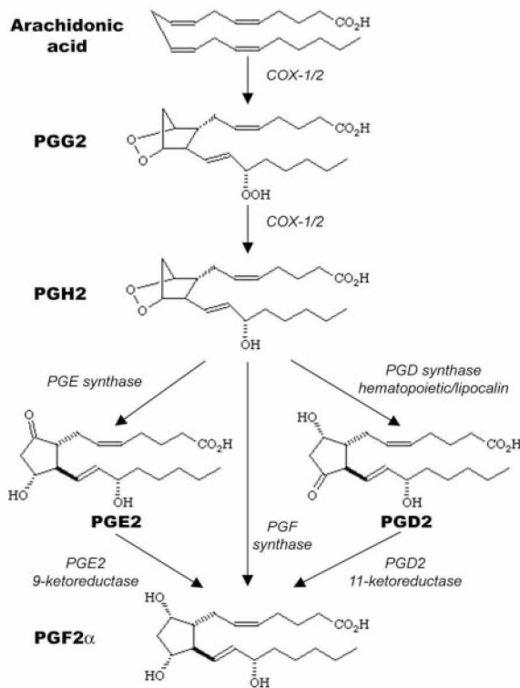
FIG. 1. Schematic representation of the COX pathway illustrating the synthesis of the major PGs. This process is initiated when COX-1 and COX-2 catalyze both a reaction in which arachidonic acid is converted to PGG 2 and a subsequent peroxidase reaction in which PGG 2 is reduced to PGH 2 , which serves as the common precursor for all of the terminal PGs.
