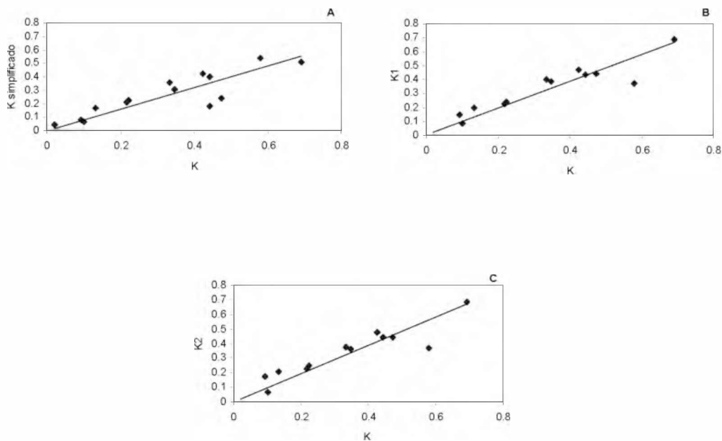
Figure 3. Lineal relationship between the erosionability factor K and simplified erosionability factor (Ks) (A) K1 (B) and K2 (C) ( t \cdot m^2 \cdot h ) ( ha \cdot J \cdot cm^3 ).
