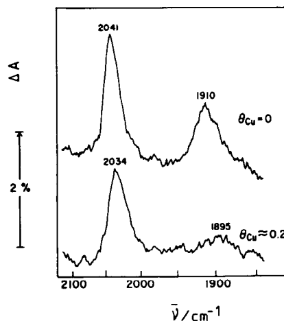
Fig. 15. Effect of underpotentially deposited Cu adatoms on the PM-IRRAS spectra of CO adsorbed on pc Rh at 0.37 V vs rhe .
