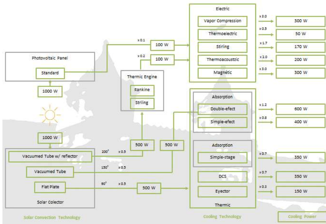
Figure 3. Performance of different technological options for solar cooling systems
