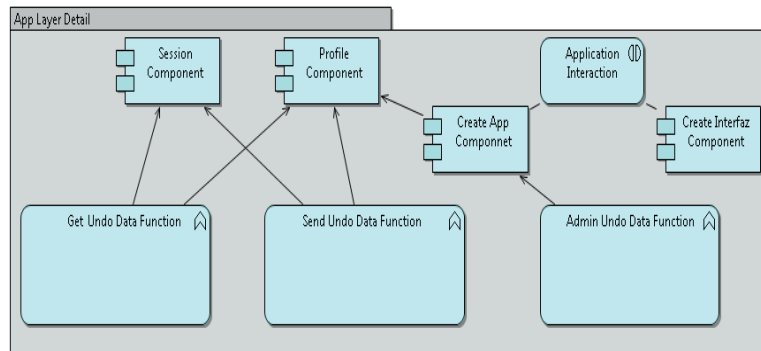
Figure 2. Undo infrastructure
