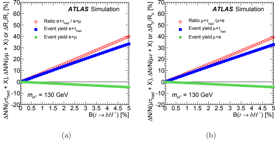
Figure 3. Relative variation with \mathcal{B}(t \rightarrow bH^+) of (a) the event yields \mathcal{N}(e + \tau_{\text{had}}) , \mathcal{N}(e + \mu) and their ratio, as well as (b) \mathcal{N}(\mu + \tau_{\text{had}}) , \mathcal{N}(\mu + e) and their ratio, assuming the presence of a 130 GeV charged Higgs boson in t\bar{t} events.
