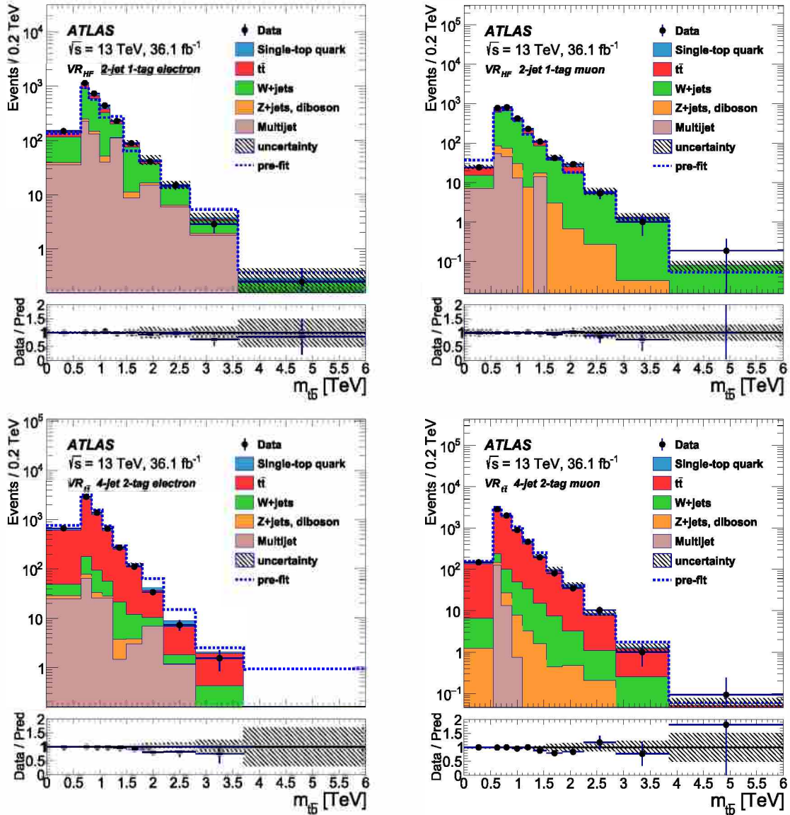
Fig. 3. Distributions of the reconstructed invariant mass of the W' boson candidate in the (top) 2-jet 1-tag VR_{HF} and (bottom) 4-jet 2-tag VR_{FT} validation regions. Background templates are fit to data in each VR using the same statistical method as for the signal region except that the normalizations of t\bar{t} and W +jets backgrounds are constrained to the post-fit rates obtained in the signal region (see Section 7). The pre-fit line presents the background prediction before the fit is performed. Uncertainty bands include all the systematic and statistical uncertainties. The residual difference between the data and MC yields is shown as a ratio in the bottom portion of each figure, wherein the error bars on the data points correspond to the data Poisson uncertainty.
