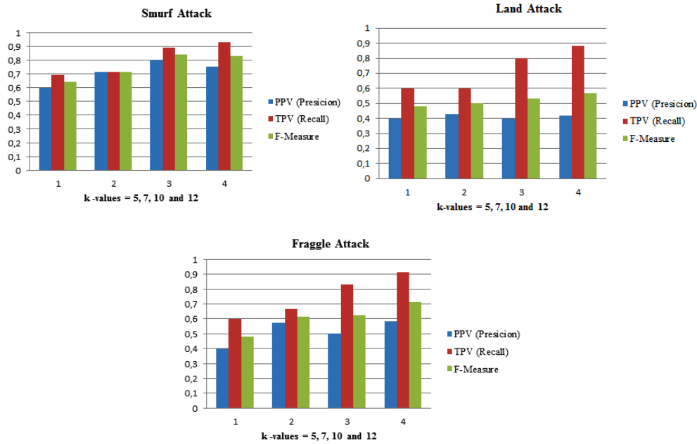
Figure 3: Results obtained in attacks: Smurf, Land and Fraggle.
