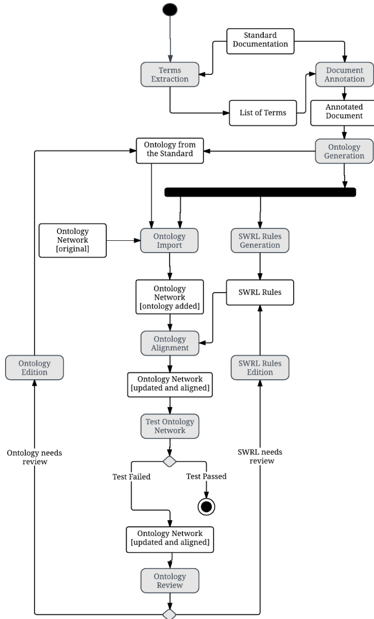
Fig.2. Activity Diagram of the Proposed Methodology
