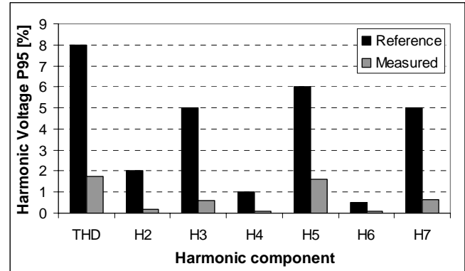
Fig. 19: Voltage harmonics reference levels and measured.
