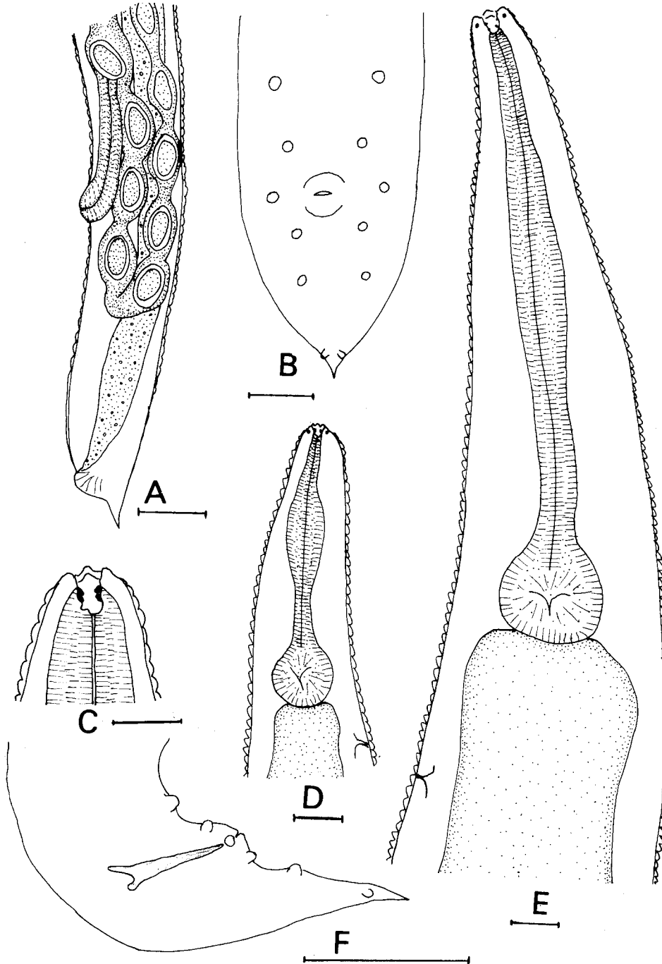
Neyraiella distinctus n. sp. A: posterior end of the female, vagina, eggs and anus; B: posterior end of the male, ventral view; C: anterior end of the female; D: stoma of the female; E: anterior end of the male; F: posterior end of the male, lateral view. Bars = 50 \mu\text{m}
