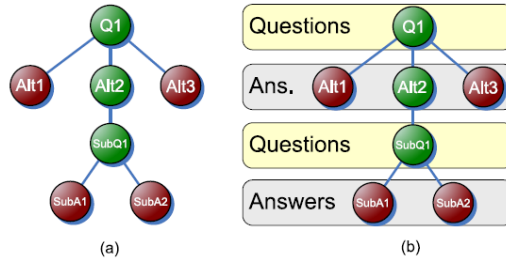
Fig. 2. Questions Tree (a) and Tree Structure (b)
