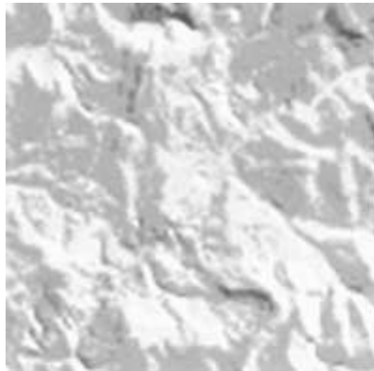
Figure 4: Shaded Relief Map.
