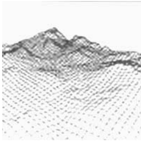
Figure 3: Pseudo 3D Projection of a land surface.
