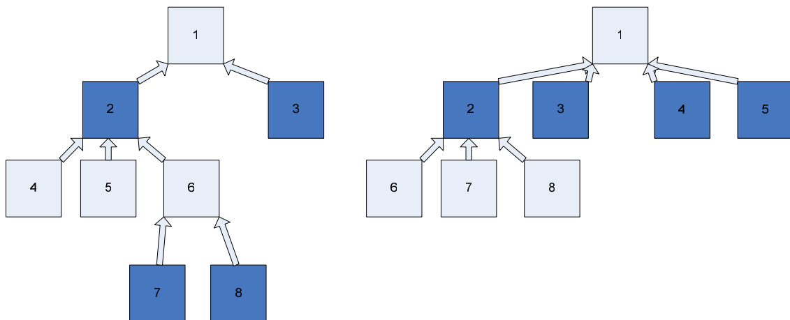
Figure 1 decision trees
