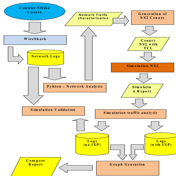
Figure 7. NS2 Methodology
