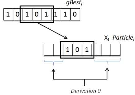
Fig. 1. Social Crossover Operator
