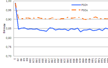
Fig. 3. PSOo and PSOh average entropy values every 20 iterations
