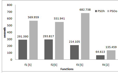
Fig. 2. PSOo and PSOh AbestT values
