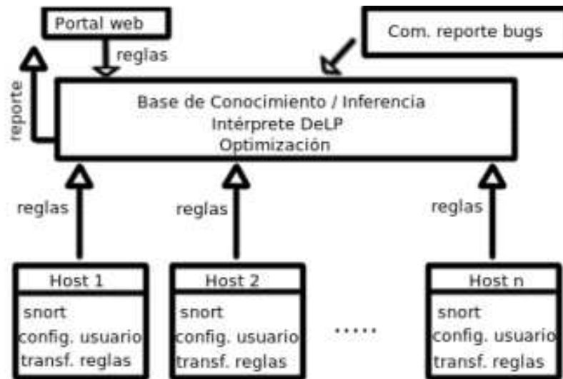
Figura 1: Framework IDS-DeLP
