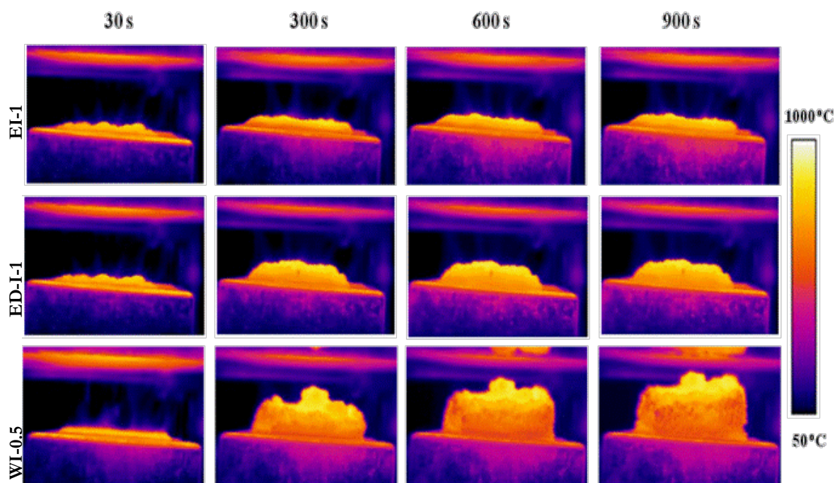
Figure 7. The intumescent char formation of EI-1mm, ED-I-1mm and WI-0.5mm during mass loss calorimetric test at 50 kW/m 2 for 900s.
