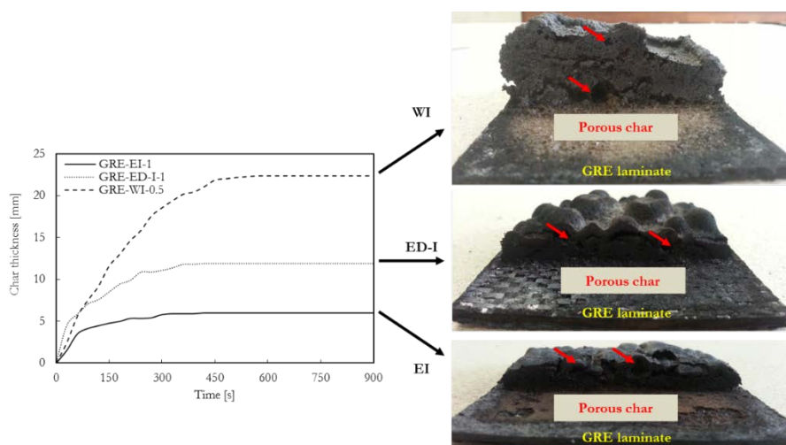
Figure 6. The char expansion vs. time curves and images of residual chars of EI, ED-I and WI intumescent coatings exposed to 50 kW/m 2 incident heat flux for 900s (part of the figure reproduced from [16]).
