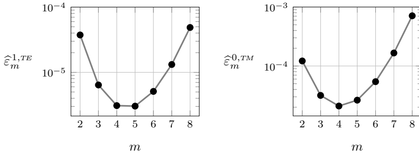
Fig. 6. Variation of \hat{\epsilon}_m^{n_s, s} \equiv \lim_{\sigma \rightarrow 0^+} \epsilon_m^{n_s}[F_\sigma^s] with m for contributions from the TE modes on the left and the TM modes on the right, calculated numerically from (5.14). For each s \in \{TE, TM\} and corresponding n_s \in \{0, 1\} , a value of m in the vicinity of a local minimum of these curves offers a potential value of M_s and a corresponding relative error |\hat{\epsilon}_{M_s}^{n_s, s} / \beta_{M_s}^{n_s, s}| for the numerical estimate of \beta_{M_s}^{n_s, s} determined in Figs. 4 and 5.
