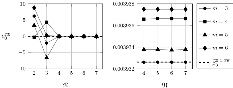
Fig. 4. Numerical values of the constant c_0^{TE} in (7.8) as a function of the largest inverse power \mathfrak{N} , derived from fitting this form to the values of \widehat{\Gamma}_m^{0,1}[F_\sigma^{TE}] given by (5.7) over the range 1/20000 \leq \sigma \leq 1/2000 for the various values of m indicated in the legend. The plot on the right indicates these variations of c_0^{TE} on an expanded scale. The numerical values of c_0^{TE} are compared with the value \widehat{\beta}_3^{0,1,TE} determined as the \sigma -independent term in the analytic series representation of \widehat{\Gamma}_m^{0,1}[F_\sigma^{TE}] in (5.18).
