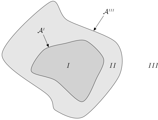
Fig. 1. Three-dimensional domains I , II and III and bounding surfaces \mathcal{A}^I and \mathcal{A}^{III} referred to in Sec. 2.
