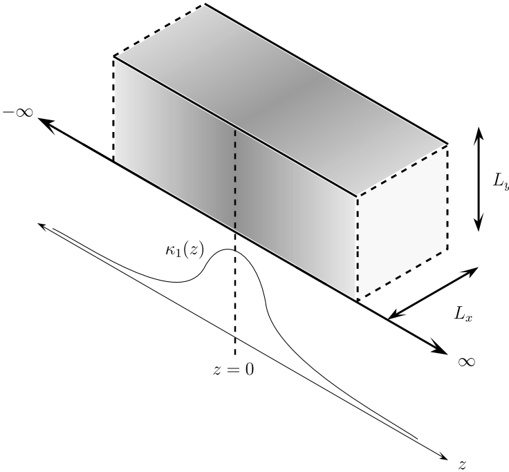
Fig. 2. Geometry of the dielectric waveguide with a smooth inhomogeneous relative permittivity profile \kappa_1(z) = \kappa_0 \operatorname{sech}^2(z/a) .
