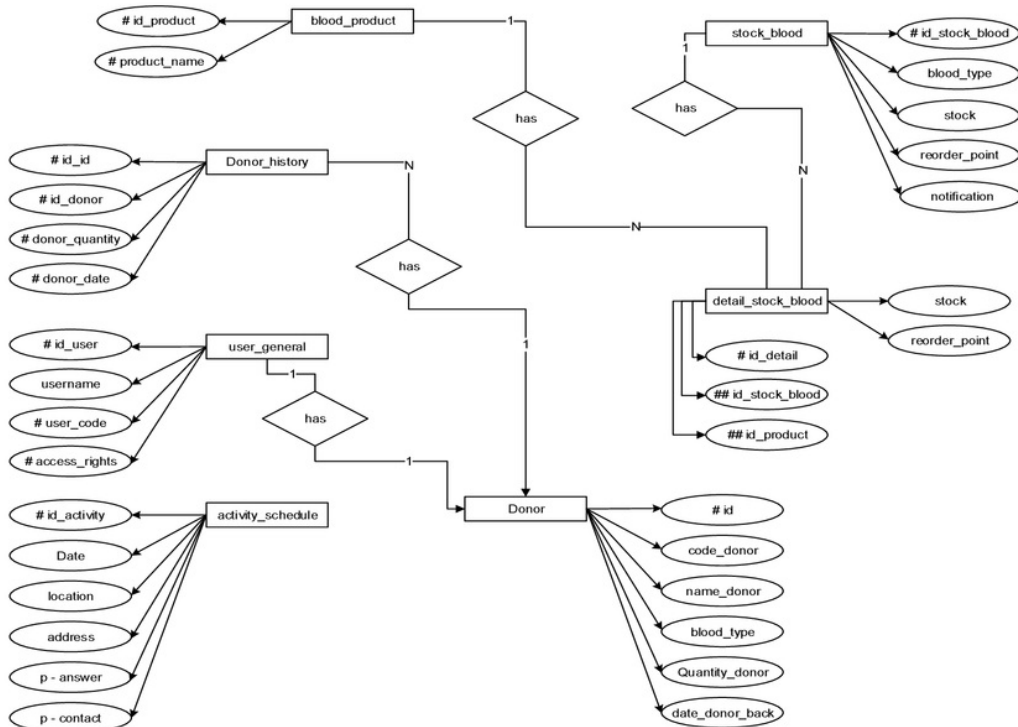
Fig 1. Entity relationship diagram
