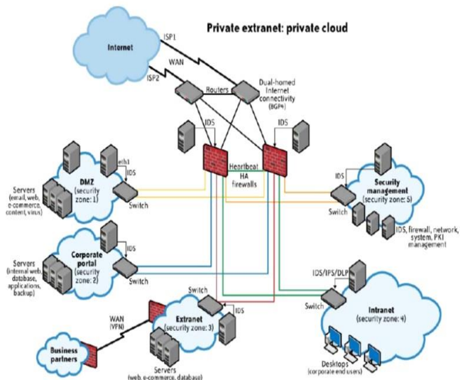
Fig 2. Generic Network Topology for Private Cloud.
