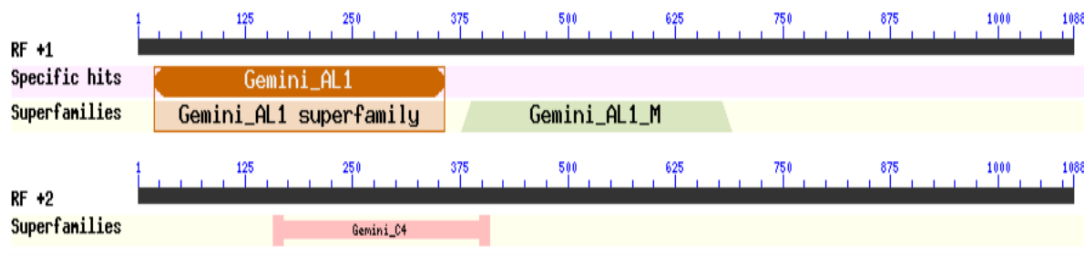
Fig 2. CD search analysis result of C1 ( Rep ) gene sequence. AL1 catalytic domain was observed at N-terminal.
