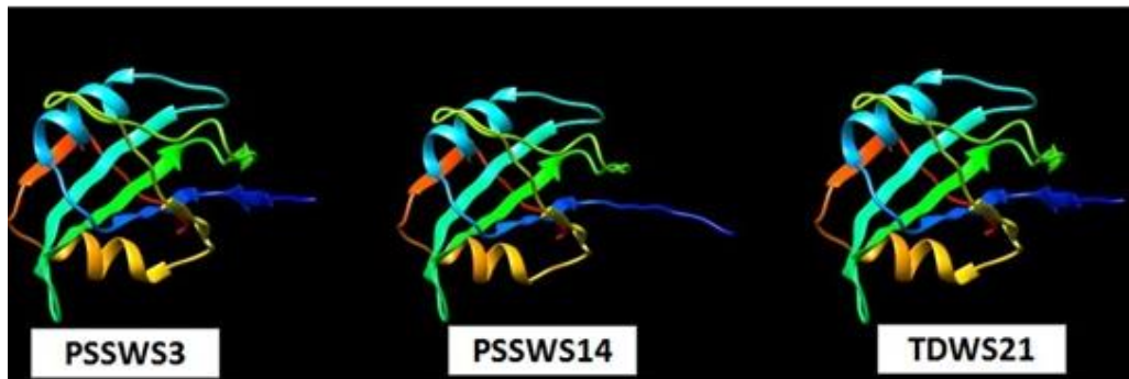
Fig 5. Modelling of three PYLCV strains. N-terminal shown in blue ribbon. C-terminal shown in red ribbon.
