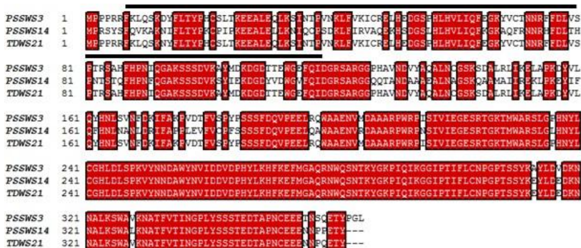
Fig 3. The full-length amino acid and alignment sequence of three PepTYLCV strains. The conserved residues are indicated by red fill box. The catalytic domain is represented by a black line.
