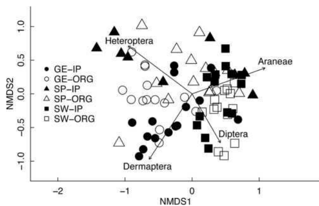
Fig. 3. Ordination of predatory arthropod communities in apple orchards in Spain (SP), Germany (GE) and Sweden (SW) for two management types: in-tegrated production (IP) and organic management (ORG). Grouping of taxa (arrows) along the two first axes of the NMDS (stress = 16.8%, 20 procrustes). Arrow length indicates the strength of predictors (taxa) fitted onto the ordi-nation for P \leq 0.001 .
