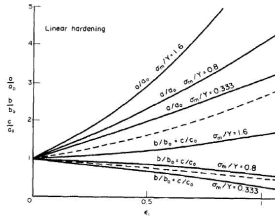
Figure 3.10 The effect of increasing plastic strain \epsilon_1 on the principal radii (a,b,c) of an originally spherical void ( a_0=b_0=c_0 ) in uniaxial tensile loading at various hydrostatic stresses ( \sigma_m/Y , Y is the yield strength for (a) non-hardening and (b) linear hardening material. The far-field loading is along the a-axis. The dotted lines show the changes in void dimensions as per the far-field strain field [Thomason, 1990].
