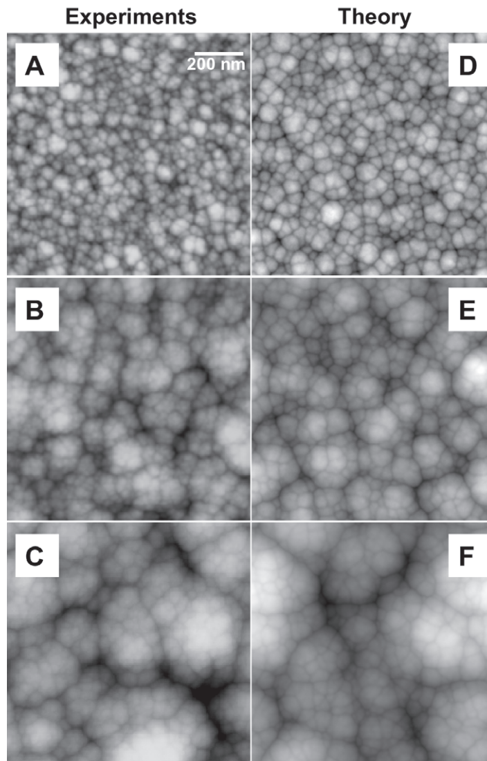
Figure 1. Nanocauliflower surface growth. AFM top views ( 1 \times 1 \mu\text{m}^2 ) of CVD experiments at times t = 40 \text{ min} (A), t = 2 \text{ h} (B) and t = 6 \text{ h} (C). Panels (D)–(F) show numerical results from equation (1) for the same times.
