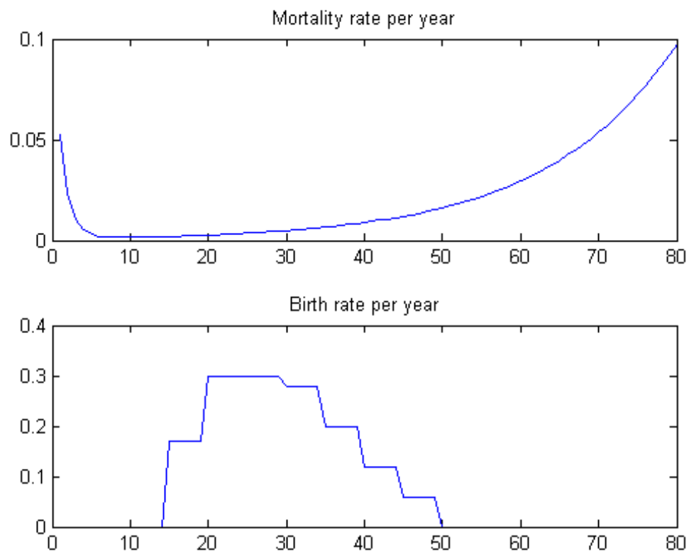
Figure 5: Mortality and fecondity as functions of age
