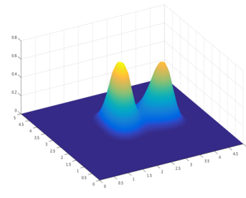
surface plot of \nu for p = 2
