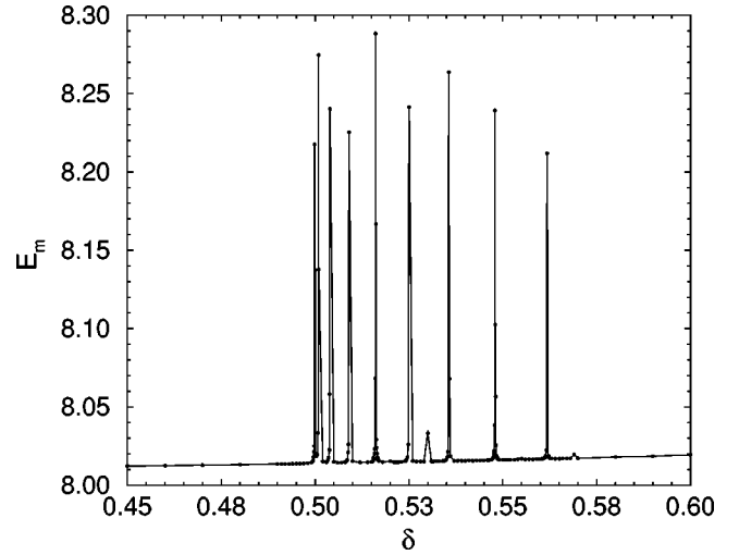
FIG. 1. Mean energy of the SG system, in dimensionless units, when \delta is close to \Omega_R/2 . Points have been calculated from numerical simulations for 10\,000 \leq t \leq 25\,000 , with \epsilon=0.01 , \delta_0=\pi/2 , u(0)=0 , X(0)=0 . The parameters of the discretization are \Delta x=0.05 , \Delta t=0.005 , and L=100 .
