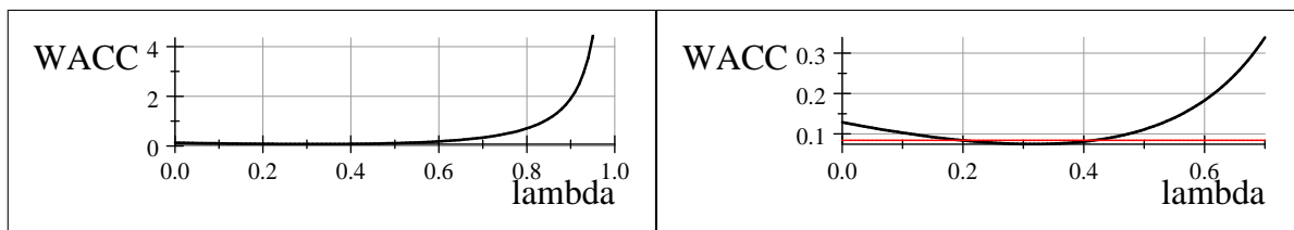
Figure 5: WACC curve
