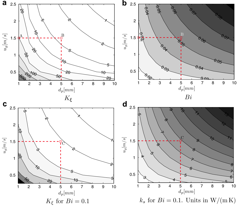
Fig. 4. (a) Non-dimensional solid conductivity in the gas flow direction K_\xi , (b) Biot number for the nominal data varying the particle size and the gas velocity; (c) and (d) represent, respectively, the non-dimensional conductivity K_\xi and the solid conductivity k_s in the limit case of Bi = 0.1 .
