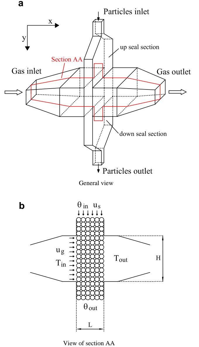
Fig. 1. Schematic of a moving bed heat exchanger (MBHE).
