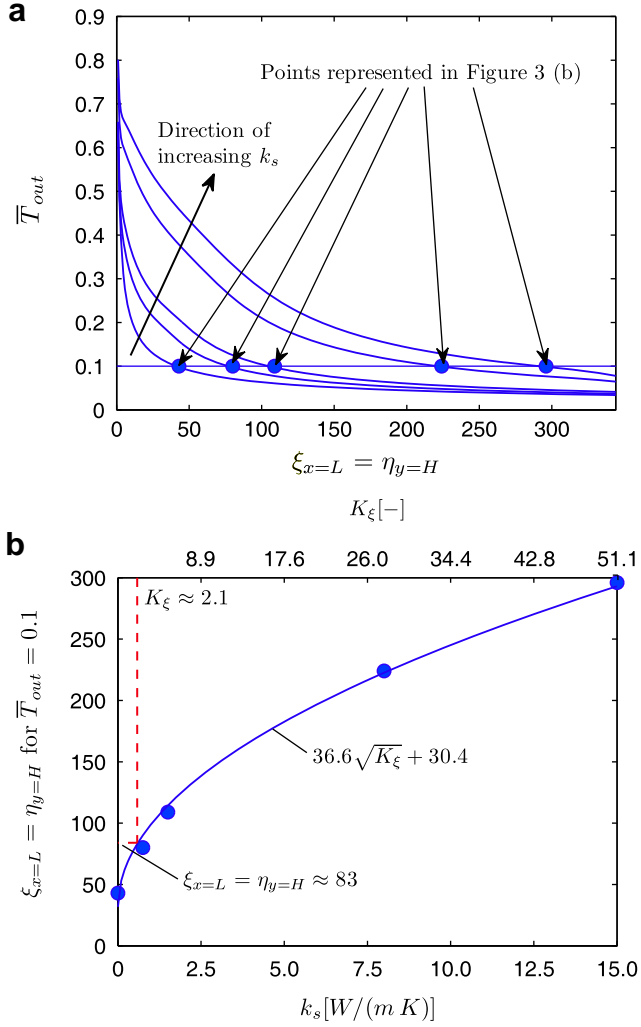
Fig. 3. (a) Non-dimensional mean outlet gas temperature for different solid conductivities ( k_s = 0, 0.75, 1.5, 8, 15 W/(mK)) and (b) \xi_{x=L} for and optimum heat exchanger ( \xi_{x=L} = \eta_{y=H} ) with an efficiency of 90% ( \bar{T}_{out} = 0.1 ) for different solid conductivities.
