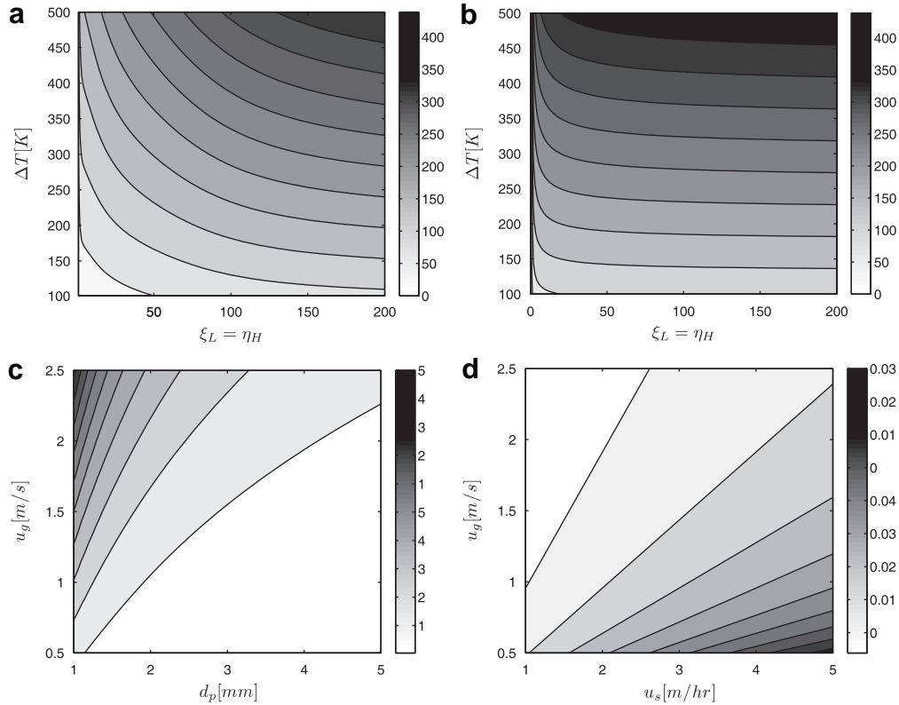
Fig. 5. (a) Heat transferred retaining solid conductivity, (b) neglecting solid conductivity for different temperature differences, (c) and (d) represent the power required to pump the gas and to raise the particles, respectively. The scale is in kJ/kg.
