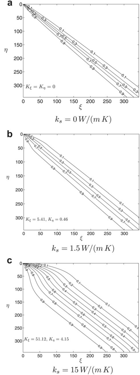
Fig. 2. Non-dimensional gas temperature profiles for the nominal MBHE. (a) Analytical solution for k_s = 0 , (b) numerical solution for k_s = 1.5 \text{ W/(mK)} and (c) numerical solution for the nominal case ( k_s = 15 \text{ W/(mK)} ).
