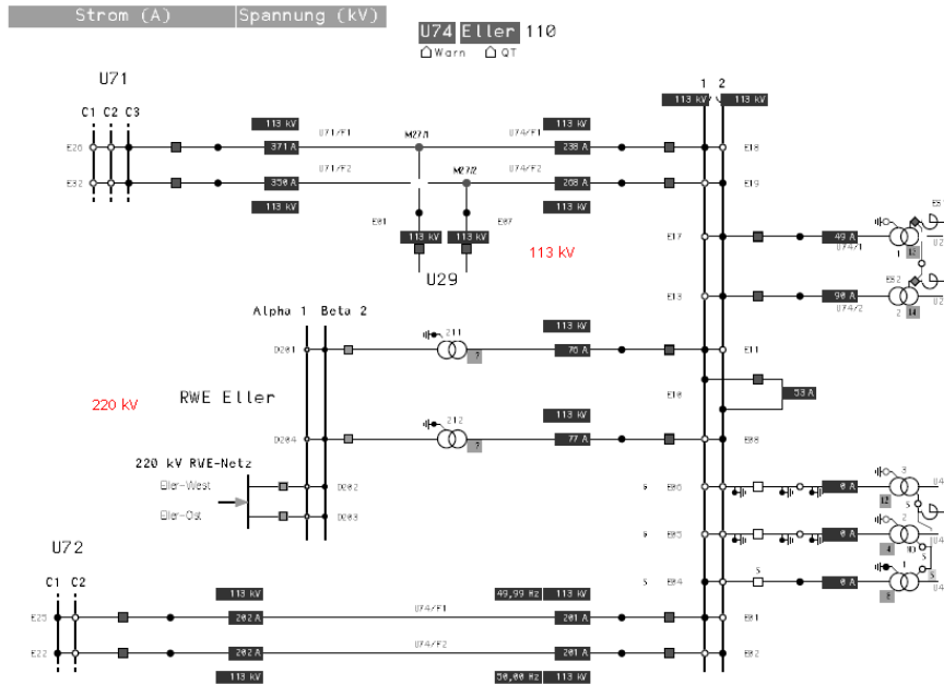
Figure 29: "220kV/110kV Network" Source: Stadtwerke Düsseldorf
