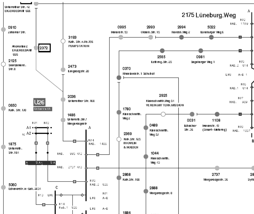
Figure 30: "10kV Grid" Source: Stadtwerke Düsseldorf
