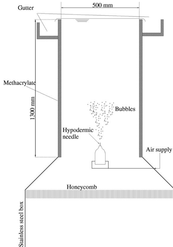
Fig. 2. Experimental set up.
