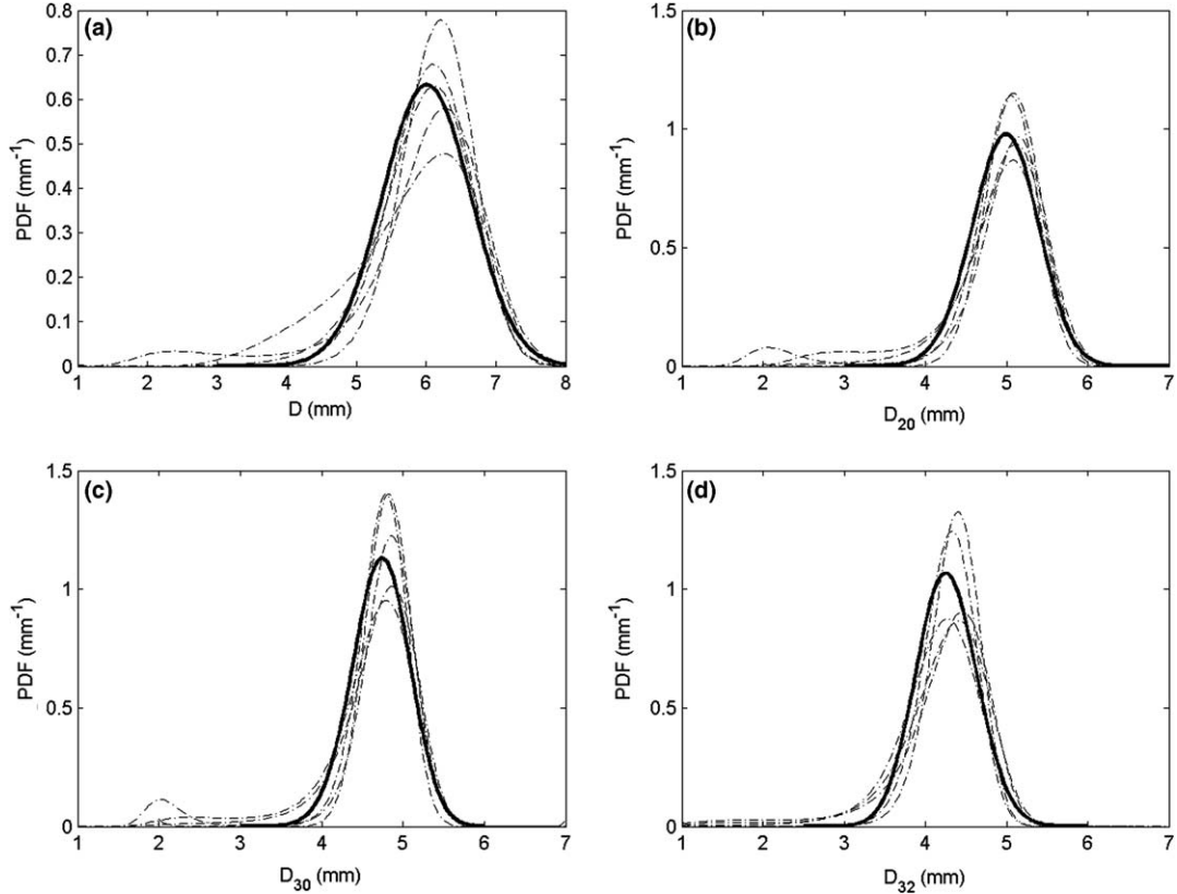
Fig. 7. Optimal MaxEnt estimation obtained from the five simulations of the chord length showed in Fig. 5, together with the experimental distribution (solid lines), for (a) bubble diameter, D , (b) surface equivalent diameter, D_{20} , (c) volume equivalent diameter, D_{30} , (d) Sauter mean diameter for five simulations, D_{32} .
