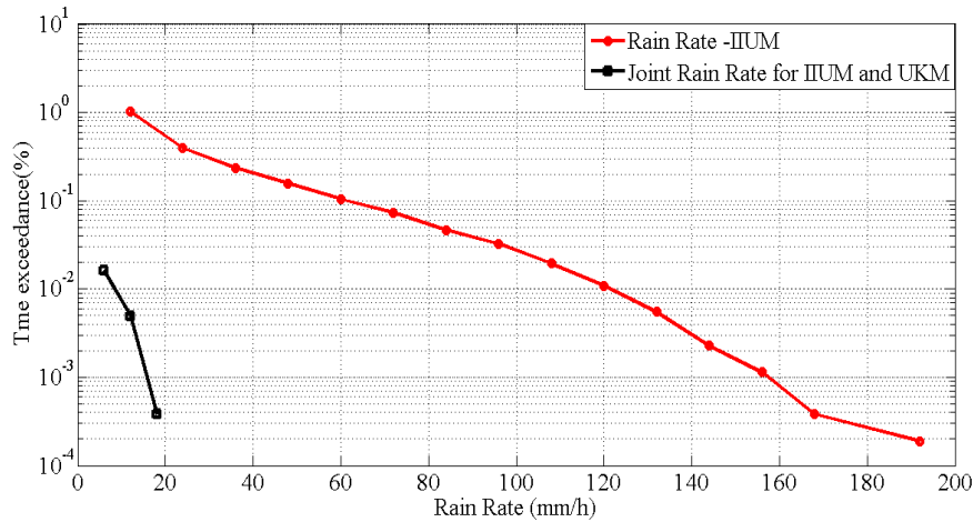
Figure 4. Cumulative Distribution Function of Rain Intensity of IIUM and Joint Distribution of IIUM and UKM Measured during 2015.
