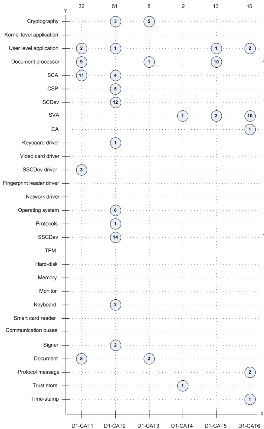
Figure 10.2: Distribution of attacks: Target versus Goal.
