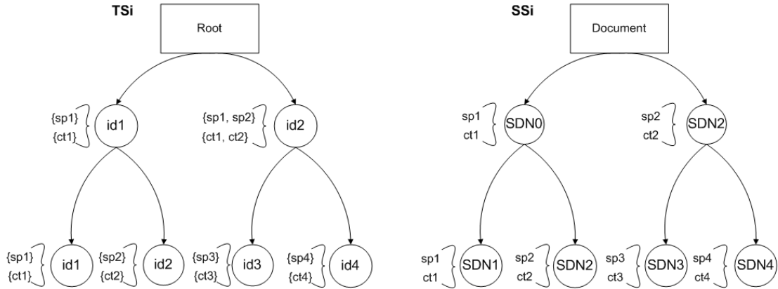
Figure 8.5: Deadlock example.
